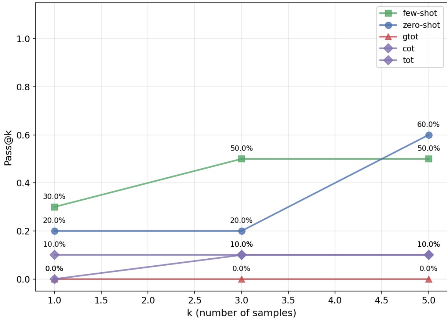
Pass@k Comparison Across Frameworks
