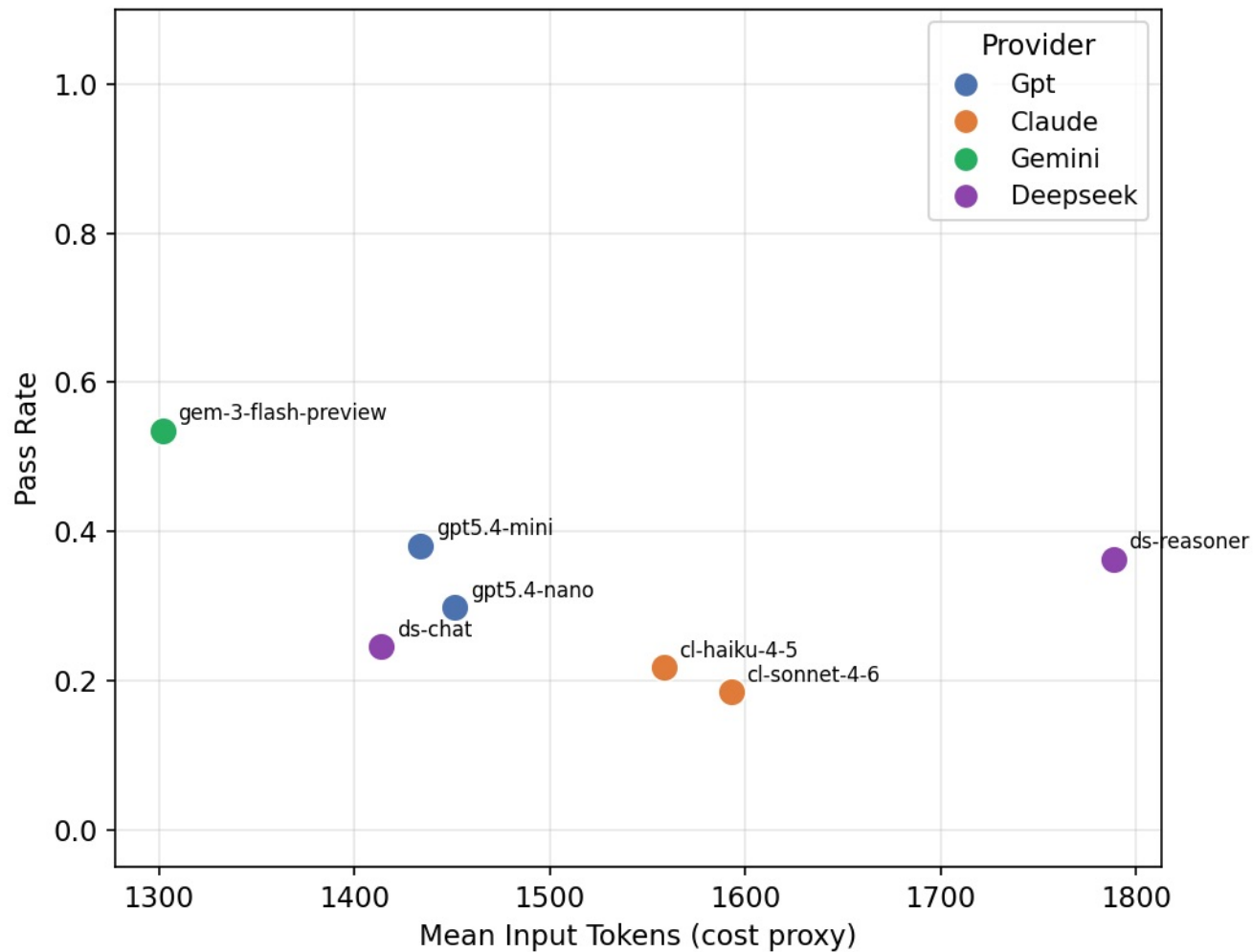
Tokens vs Pass Rate
