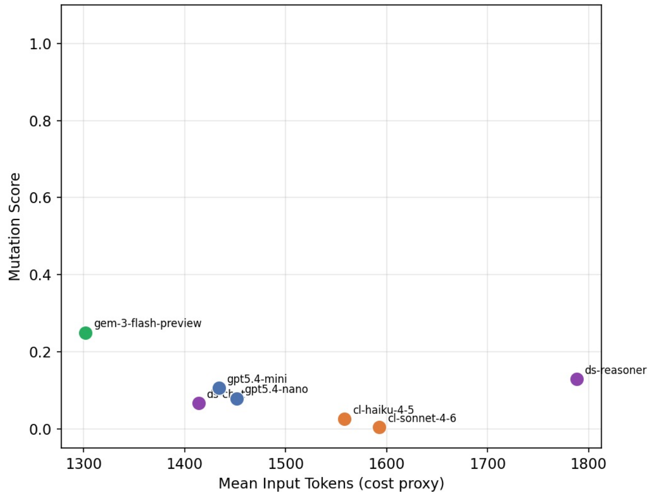
Tokens vs Mutation Score
