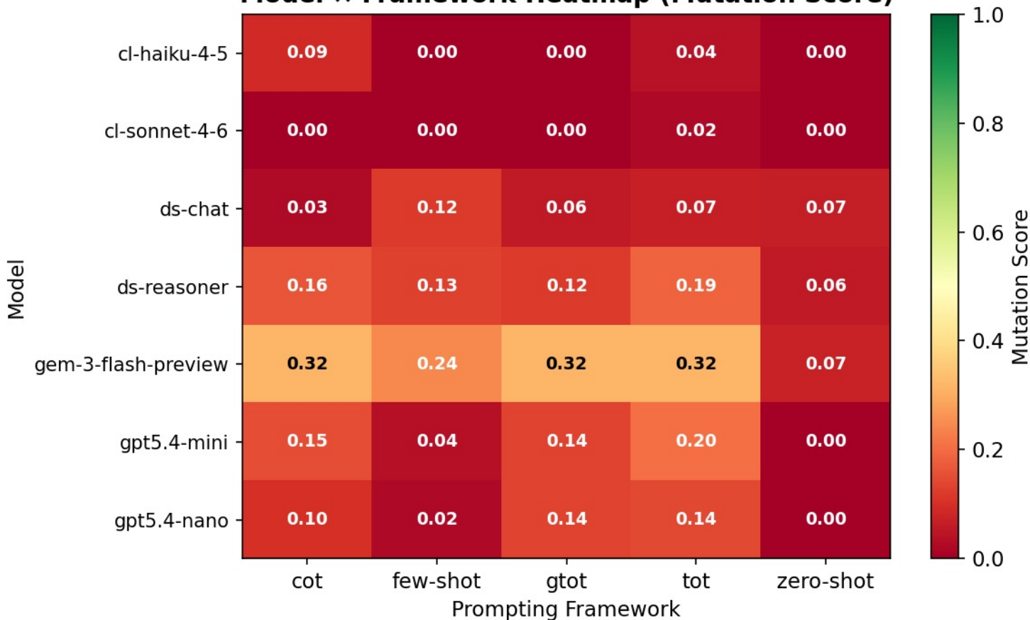
Model × Framework Heatmap (Mutation Score)
