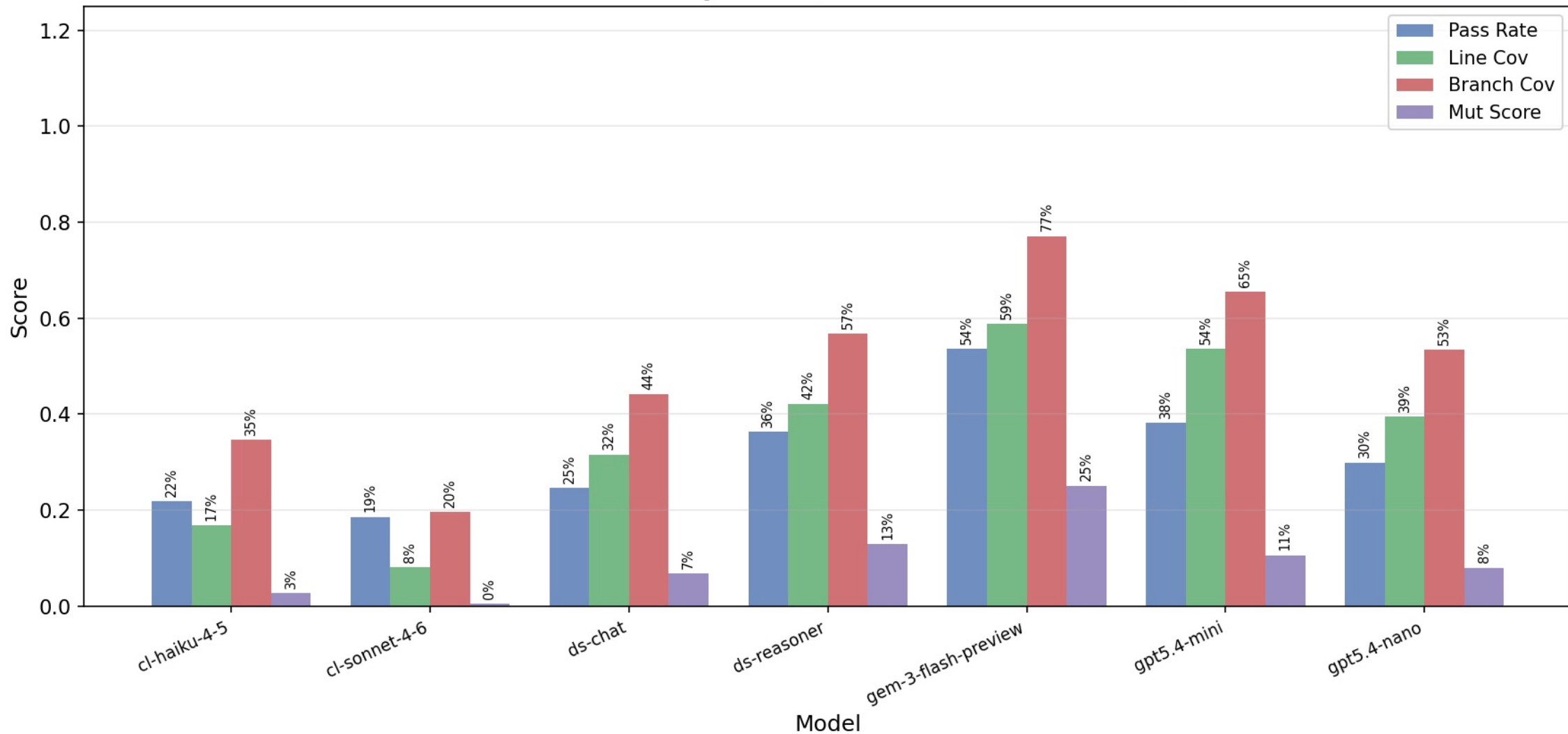
Cross-Model Comparison (all frameworks & k values)
